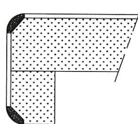
GEM-LOCK EDGE; LAMINATE TOP AND EDGE WITH 1/4" SOLID SURFACE QUARTER ROUND INLAY TOP AND BOTTOM
