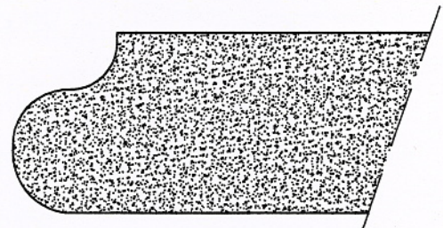
CUSTOM OGEE BULLNOSE
